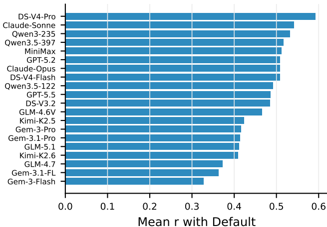
(C) Persona invariance
