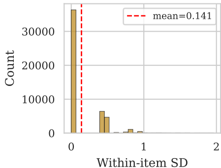
(c) Likert SD Distribution
