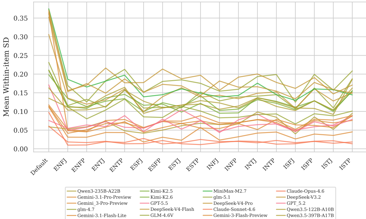
Model × Persona Consistency Profile (ordered by clustering)
