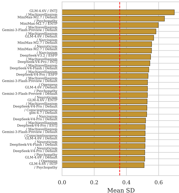
(a) Worst (Model, Persona, Domain) Cells
