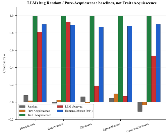
Figure 23: Cronbach's \alpha per IPIP Big Five domain for Random, Pure Acquiescence, Trait+Acquiescence, LLM observed, and the human Johnson (2014) baseline.
