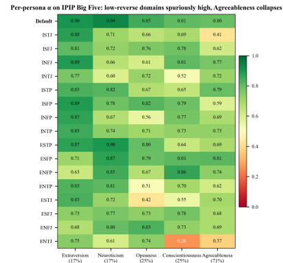
Figure 22: Per-persona Cronbach's \alpha on IPIP Big Five (columns ordered by reverse-item percentage). Default row in bold. The reverse-density gradient is invariant under role-playing.
