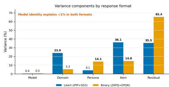
Figure 5: Sequential variance decomposition. Inter-model variance: 0.35% (Likert), 0.51% (Binary).
