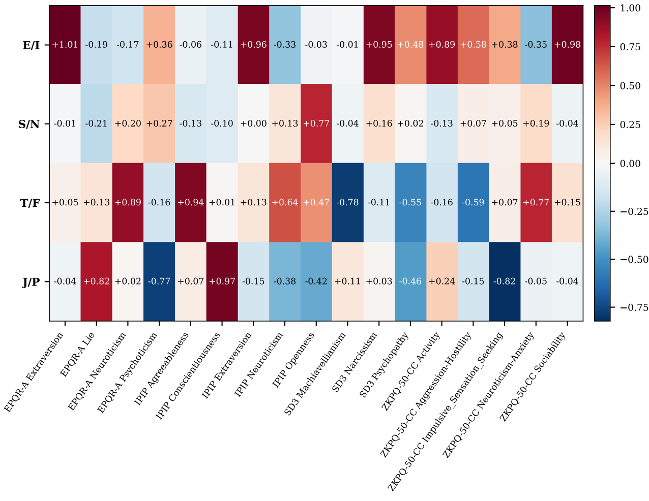
Factorial MBTI main effects (standardized \beta ) on the 17 domain scores
