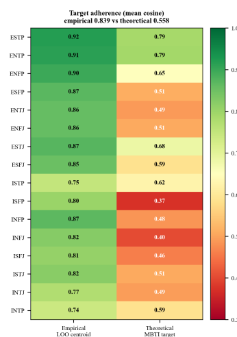
Figure 12: Per-persona target adherence: LOO-empirical (left column) vs theoretical MBTI mapping (right column).
