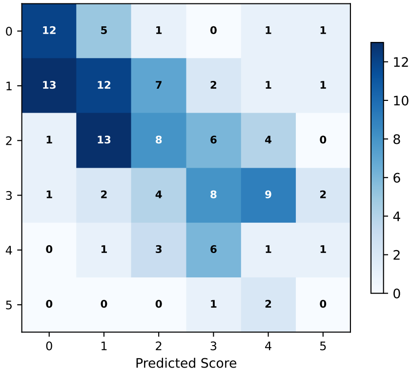
RewriteJudge (Qwen3-8B) (Counts)
