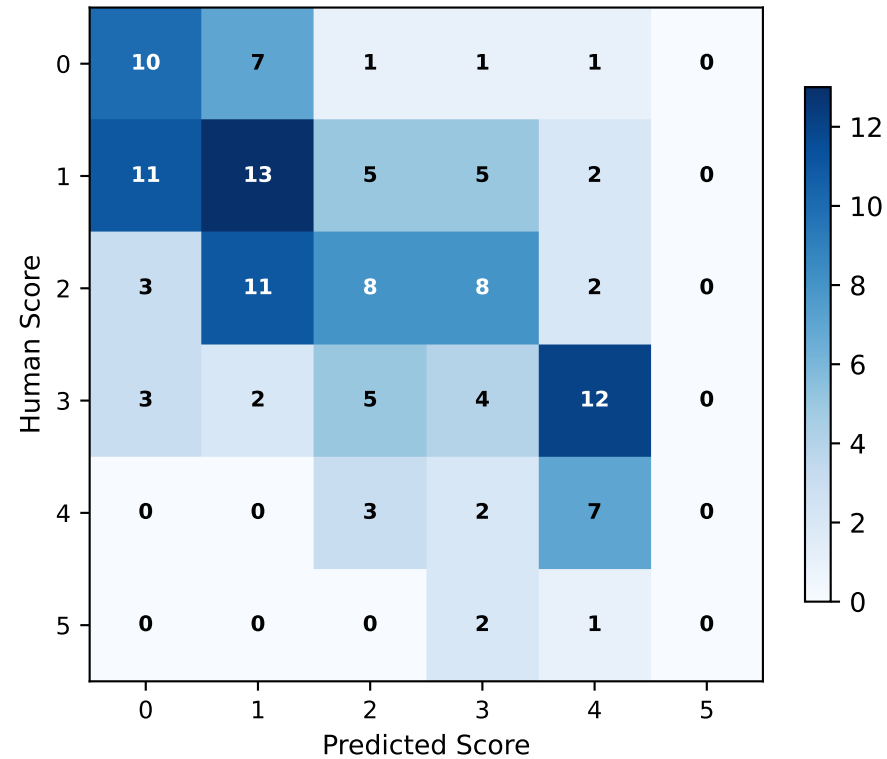
RewriteJudge (Qwen2.5-7B) (Counts)
