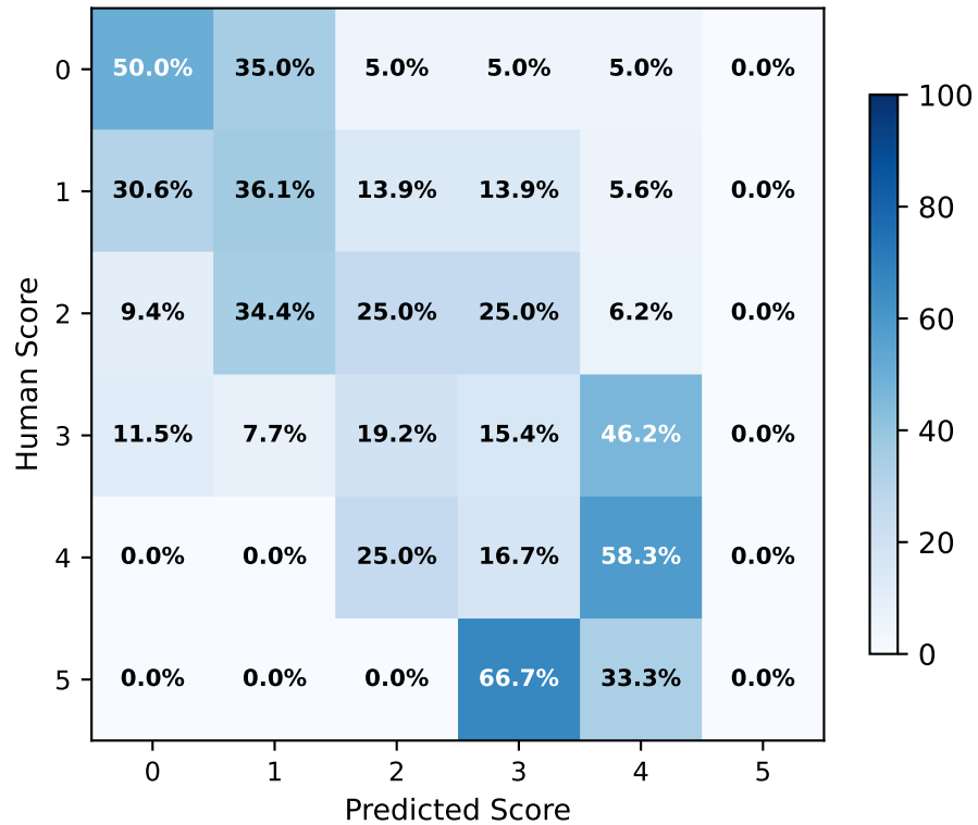
RewriteJudge (Qwen2.5-7B) (Row-normalised (%))
