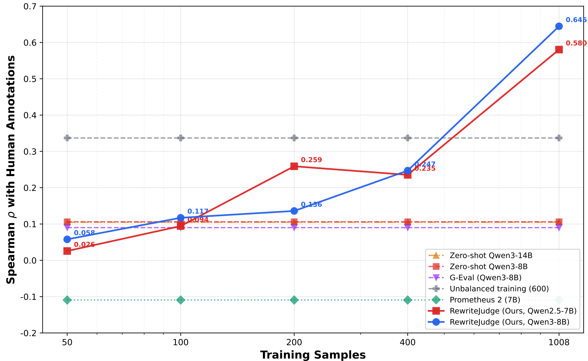
Learning Curves: Evaluator Performance vs Training Data Size
