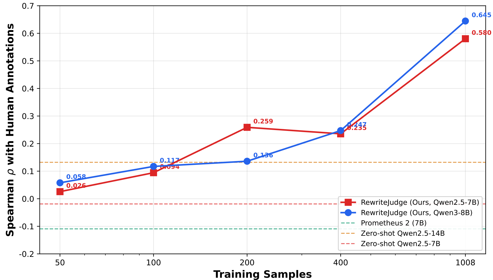
LoRA Evaluator Learning Curve
