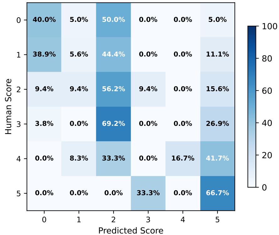
RewriteJudge-400 (Row-normalised (%))
