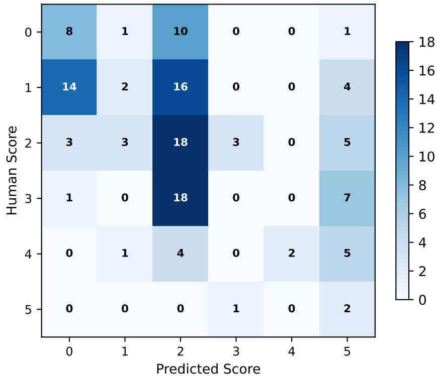
RewriteJudge-400 (Counts)
