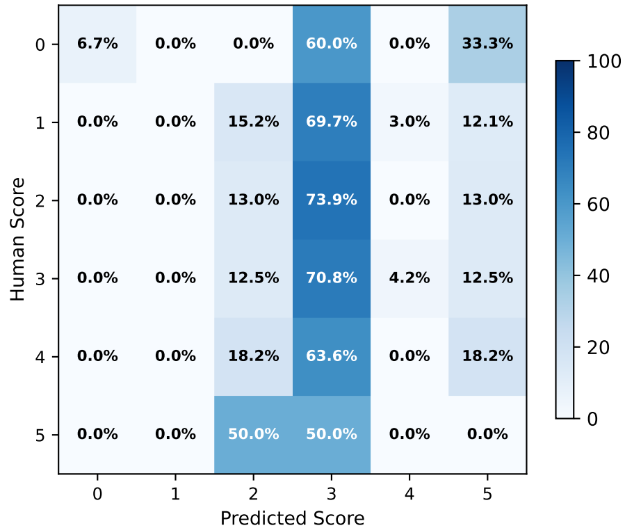
Prometheus 2 (Row-normalised (%))
