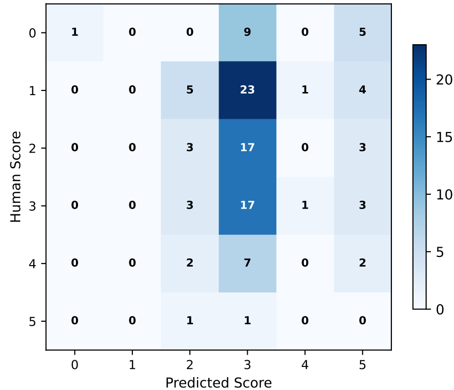
Prometheus 2 (Counts)
