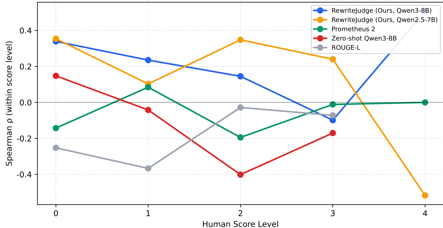
Per-Score-Level Evaluation Quality
