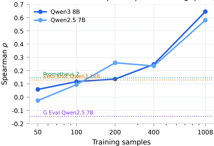
More balanced examples improve ranking quality
