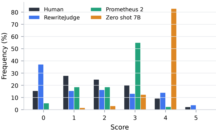
Balanced training avoids score collapse
