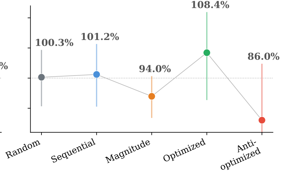
RoBERTa-InBedder
