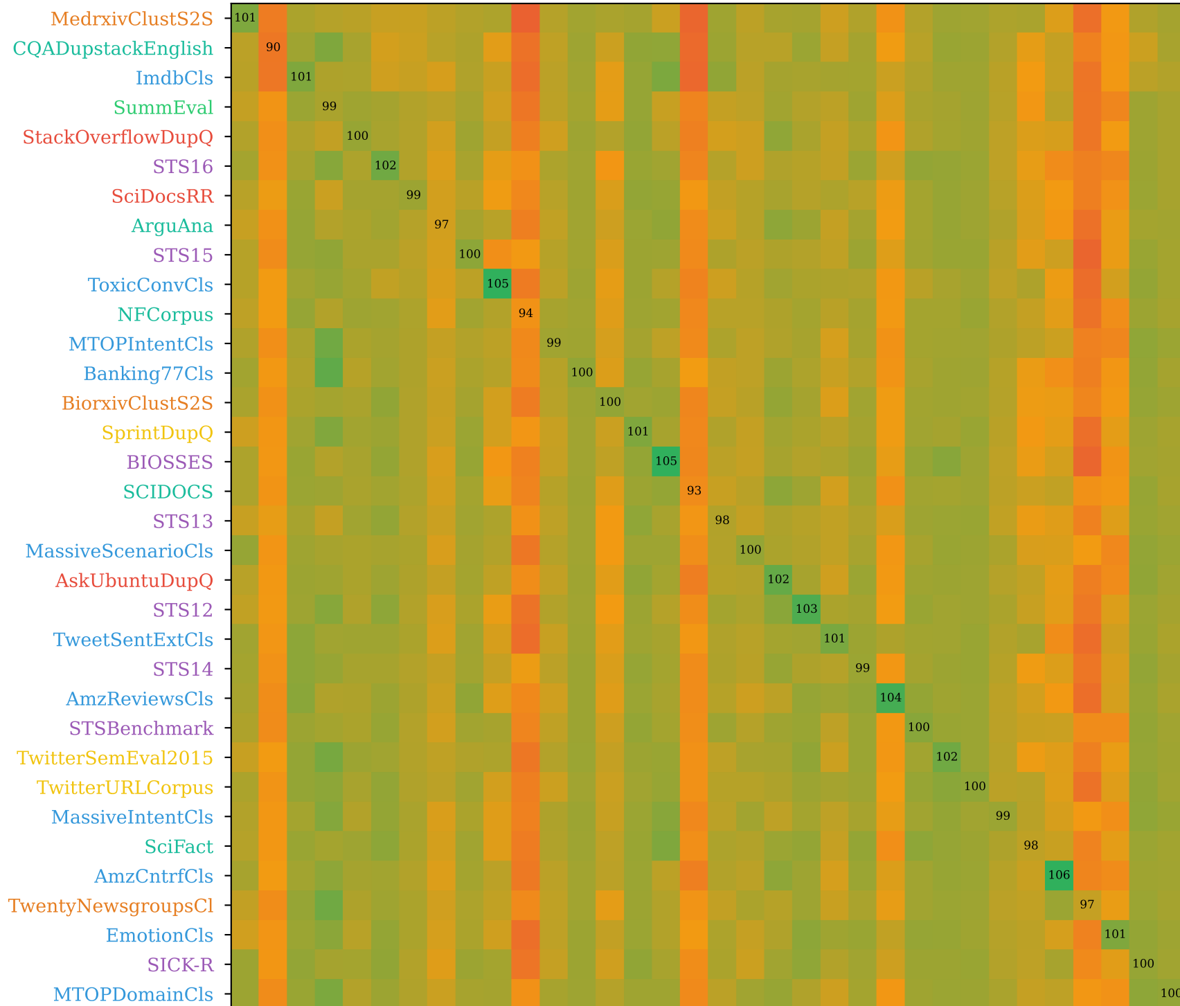
GTE-Large Cross-Task Dimension Importance Transfer
