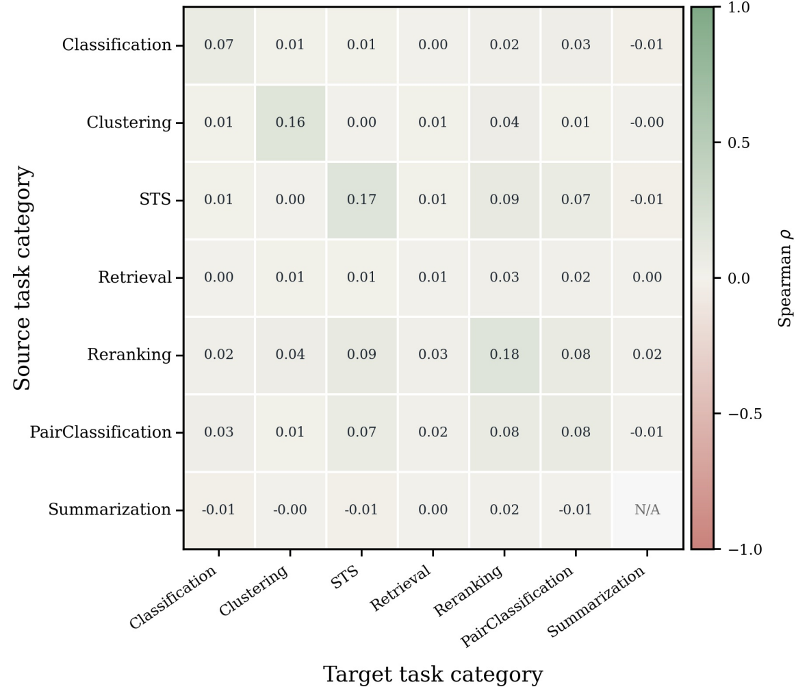
(b) Cross-Task Rank Correlation
