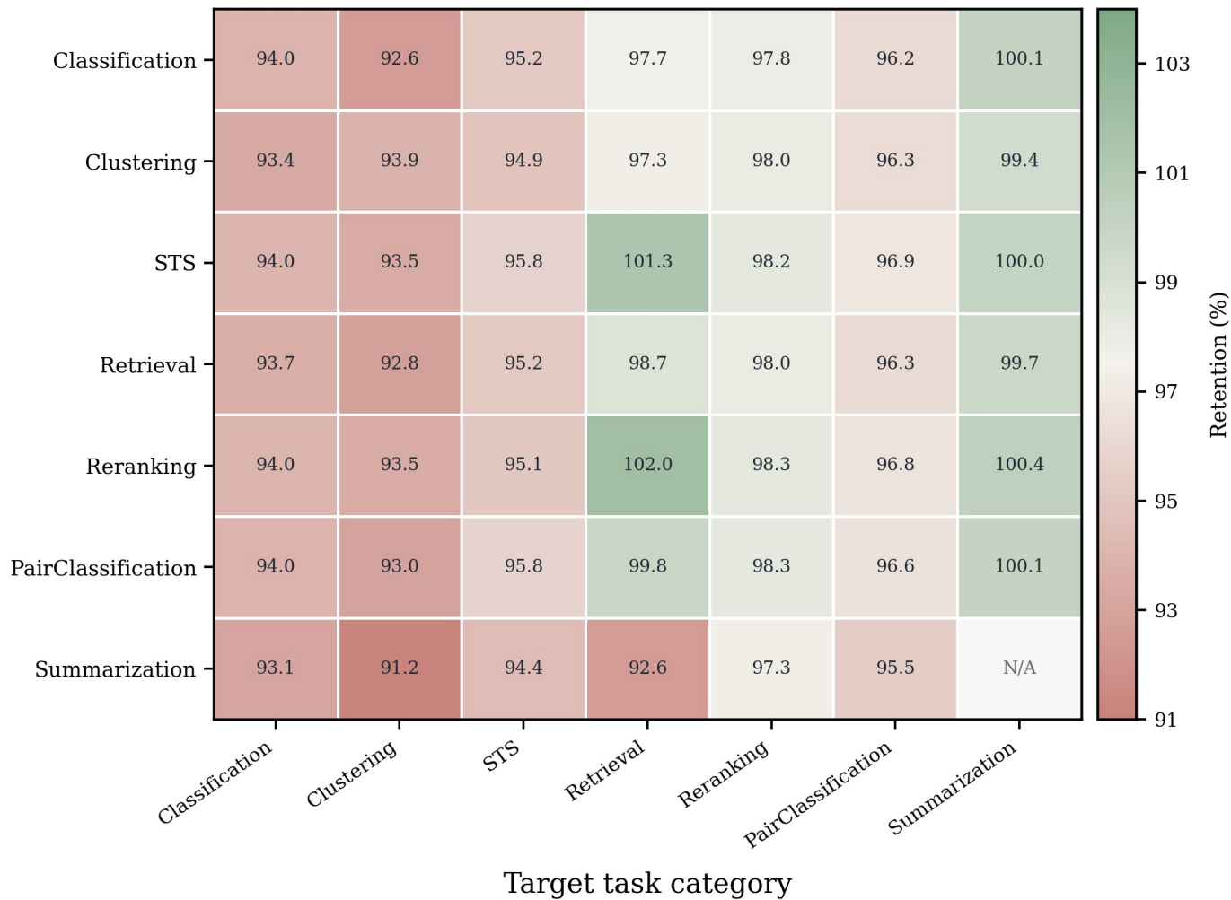
(a) Category-Level Cross-Task Transfer
