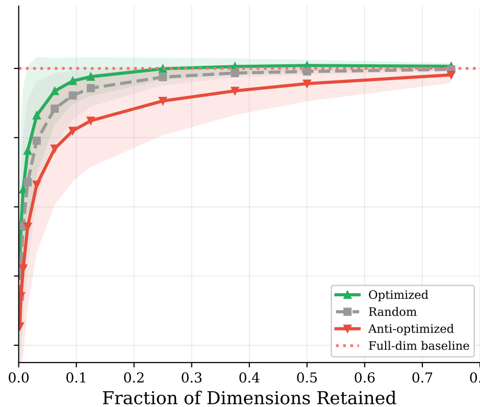
GTE-Large (1024d)
