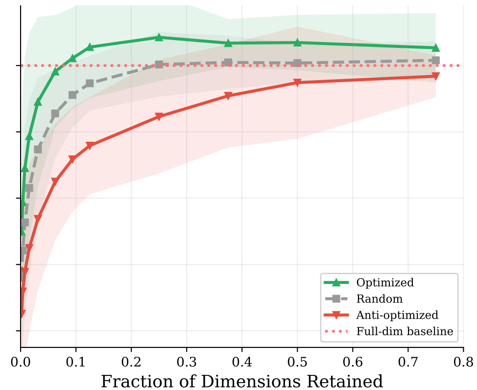
RoBERTa-InBedder (1024d)
