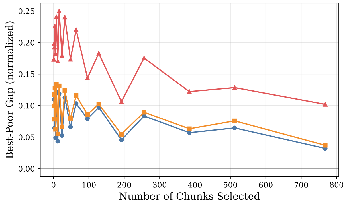
(b) Selection Quality Gap (three focal models)
