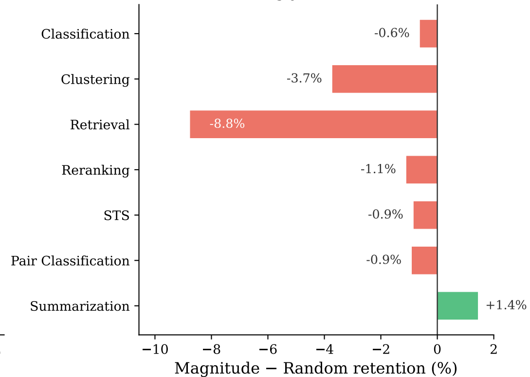
(c) Failures concentrate most strongly on retrieval
