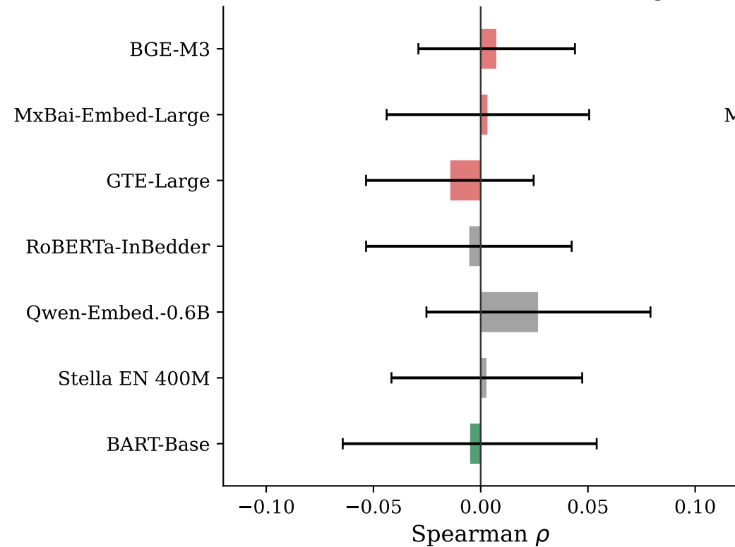
(a) Weight magnitude is nearly uncorrelated with task ranking
