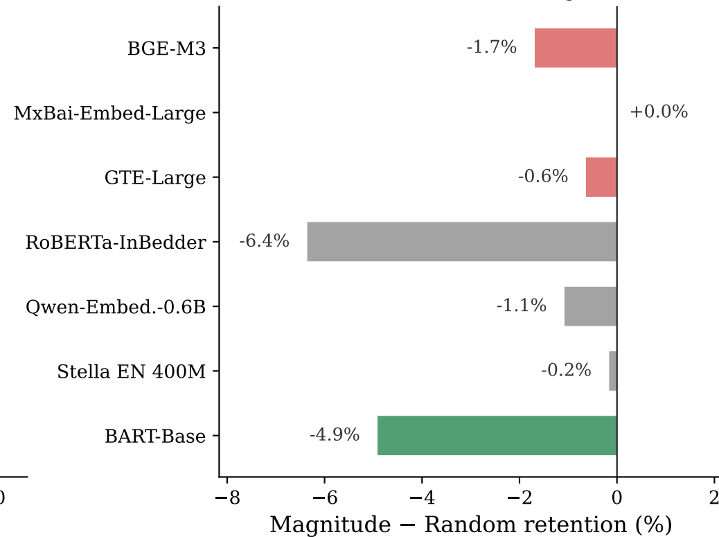
(b) Magnitude does not provide a reliable retention gain
