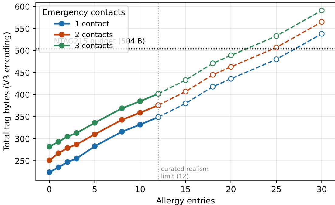
Payload size vs. allergy count and contact count (V3)
