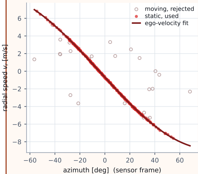
Radar detections paper front end one scan, 310 returns, 92% inliers, residual 0.036 m/s
