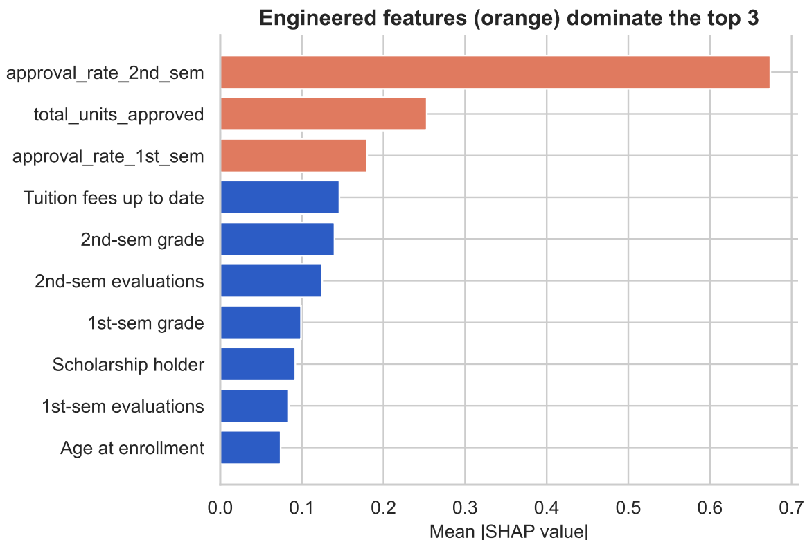
Figure 6: Top 10 features by mean |SHAP value| — the engineered trajectory features dominate.
