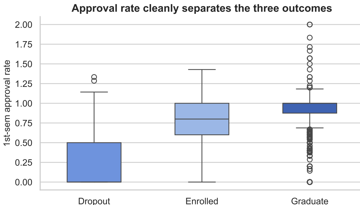
Figure 2: 1st-semester approval rate by eventual outcome — the gap between Dropout and Graduate is exactly the signal this engineered feature was designed to expose.
