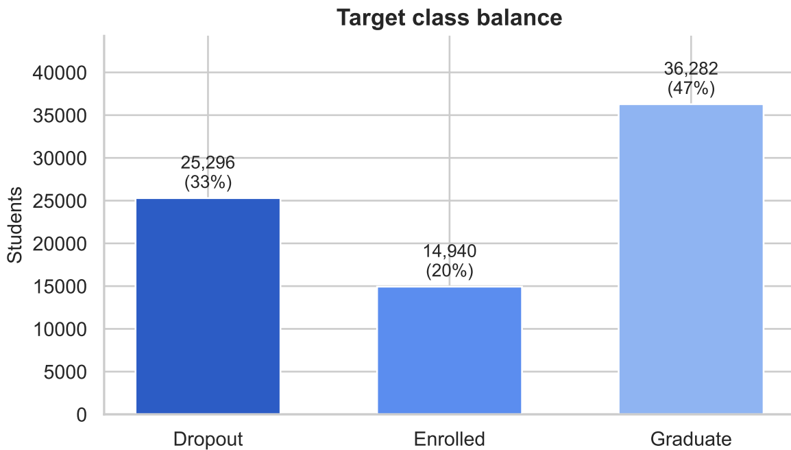
Figure 1: Target class distribution across the 76,518-row training set.
