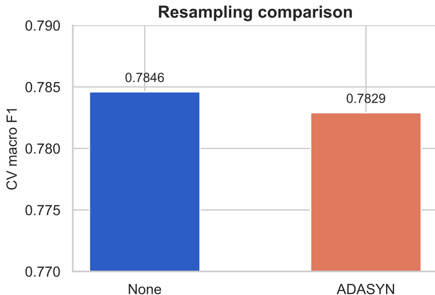
Figure 4: ADASYN oversampling slightly hurt macro-F1 on this dataset.
