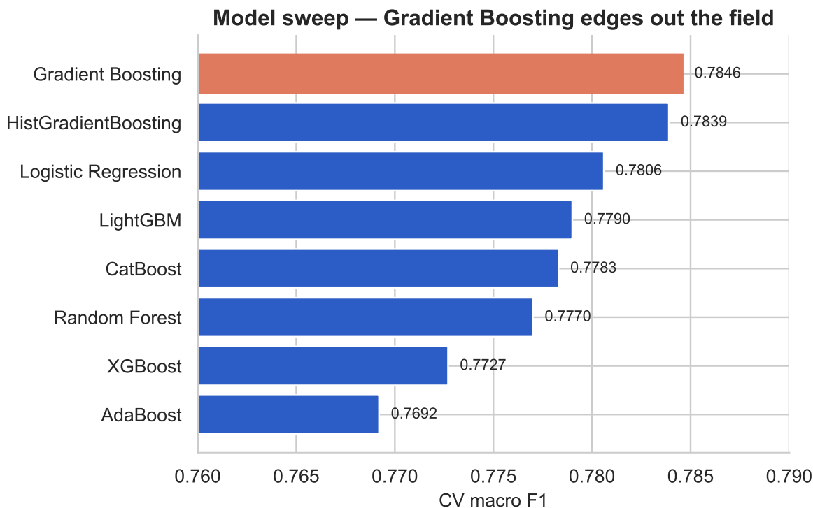
Figure 3: Cross-validated macro-F1 across all 8 model families (15,000-row subsample).
