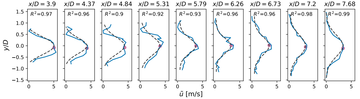
FIG. 9: Detected wake centers showing Gaussian fit against momentum deficit. Blue lines indicate momentum deficit estimated from lidar scans, dashed line shows the fit Gaussian profile, point marker is the detected wake center \mu/D .
