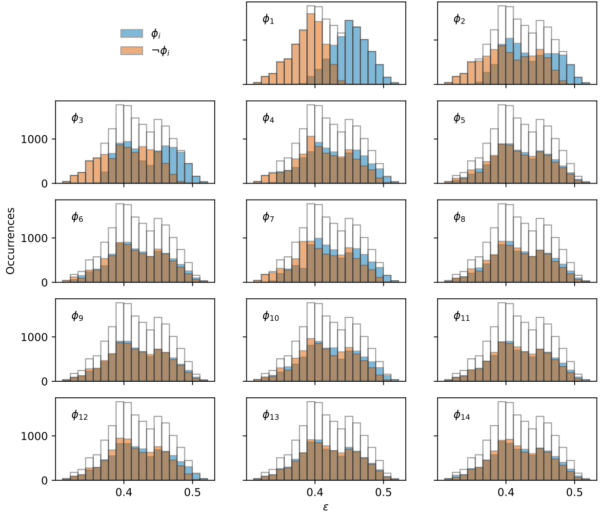
FIG. 20: Distributions of \varepsilon consider ROMs that include each mode (blue) or exclude each mode (orange).
