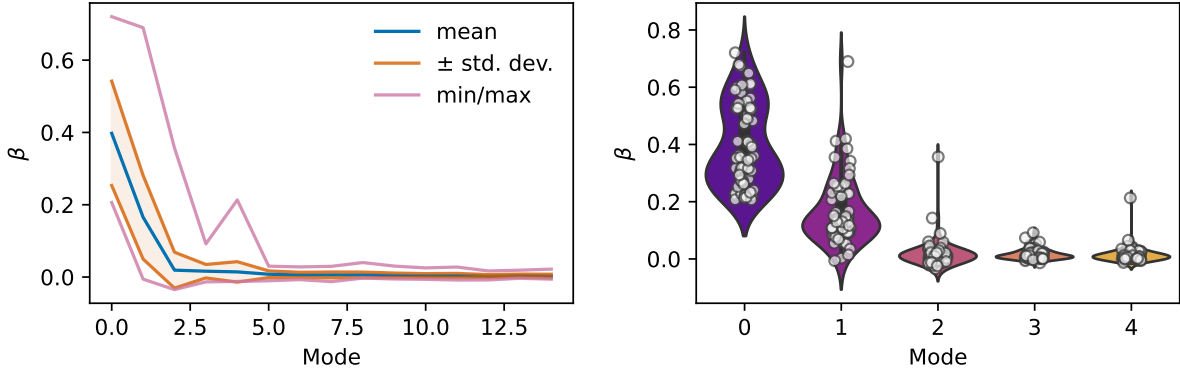
FIG. 23: Trends of \beta considering all 65 cases in the overall study. Correct mode indices for both subplots. Should begin at 1...
