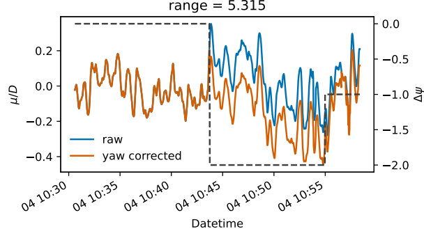
FIG. 8: Detected wake centers directly from lidar observations (blue) and after correcting for yaw activity of the turbine (orange). The dashed black line indicates nacelle position changes from the beginning of the time series and corresponds with the axis labels on the right.
