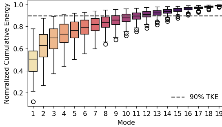
FIG. 13: The distribution of cumulative TKE described by the POD eigenvalues for the collection of 65 cases.
