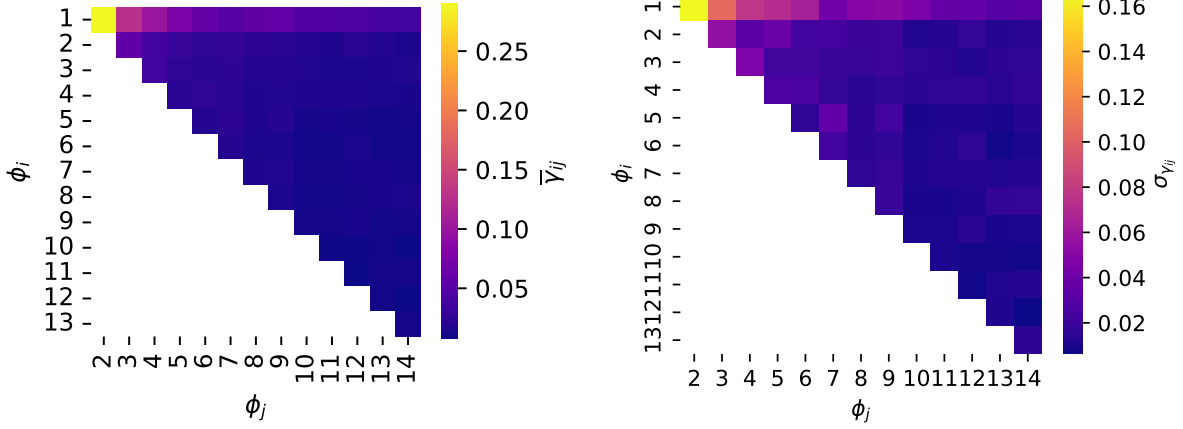
FIG. 24: Trends of \bar{\gamma}_{ij} = f(\phi_i, \phi_j) considering all 65 cases in the overall study. Does gamma only show absolute values??
