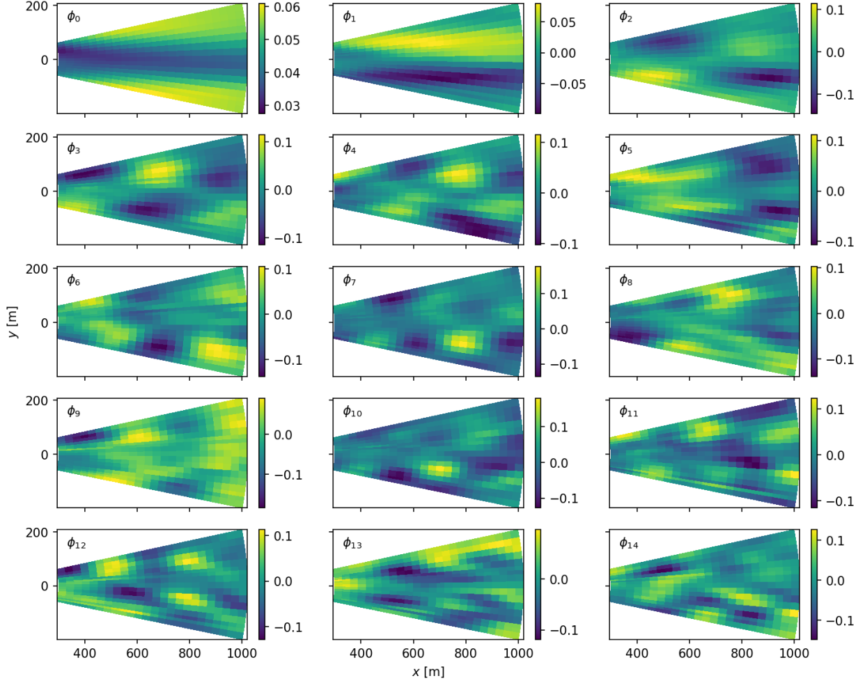
FIG. 14: POD modes from the example case on 2023-09-04 10:30 UTC.
