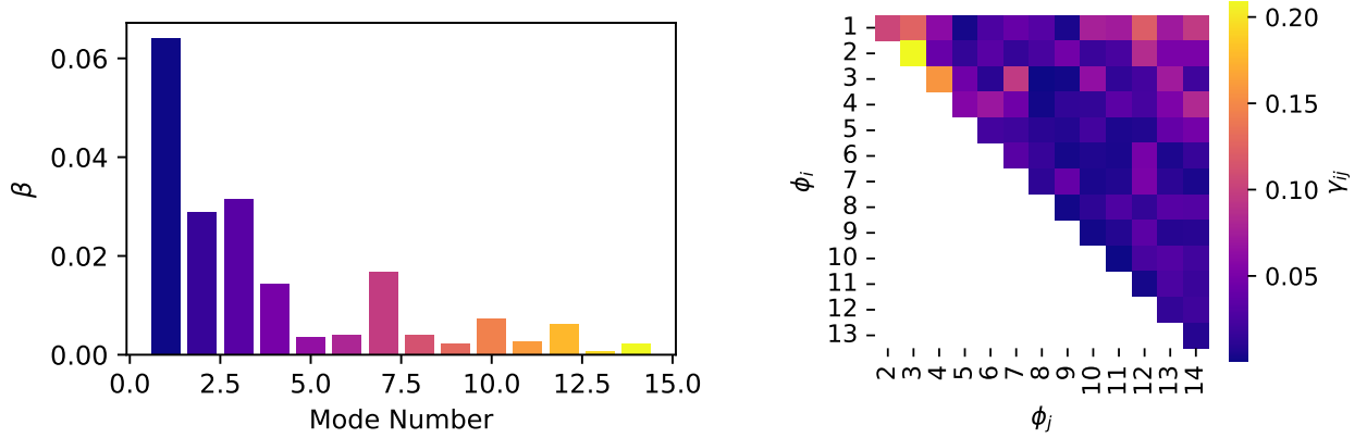
FIG. 19: Main effect \beta_i of each mode and interaction effects \gamma_{ij} between modes building the linear system that describes the dependence of average coherence on the presence or absence of each mode. Check that \gamma is not shown only absolute values. Some of the interaction effects should be negative.
