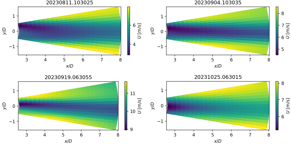
FIG. 6: Average wake velocity fields for 2023-08-11 10:30 (top left), 2023-09-04 10:30 (top right), 2023-09-19 06:30 (bottom left), 2023-10-25 06:30 (bottom right) showing a range of background velocities, momentum deficits and wake recovery rates.
