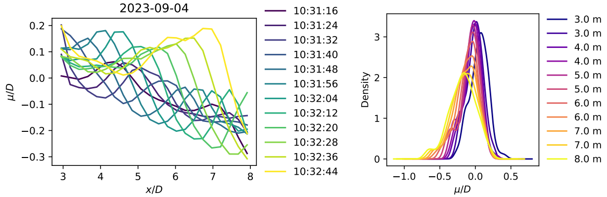
FIG. 11: Wake center trajectories for selected times (left) and kernel density estimates of wake centers by distance downstream of the lidar (right).
