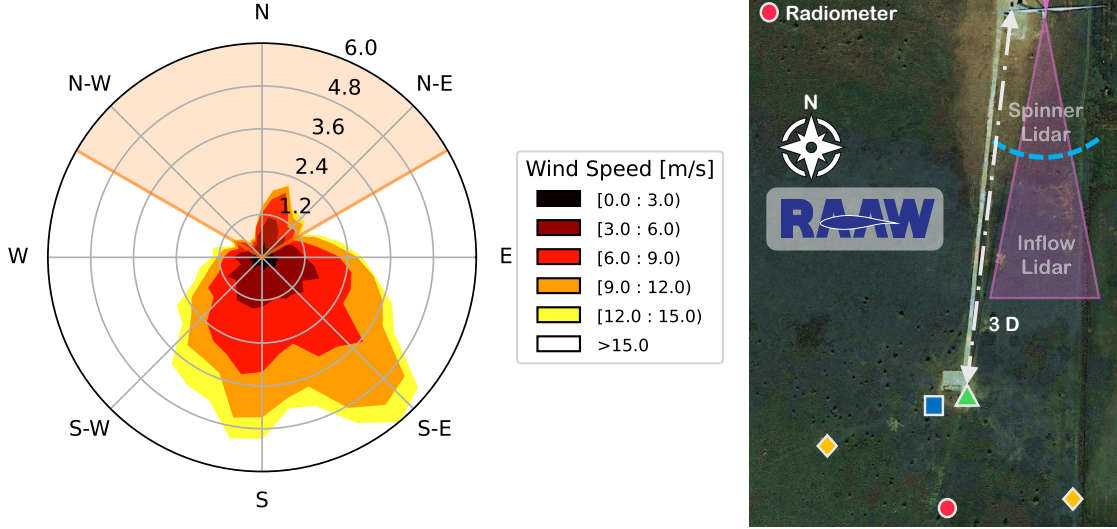
FIG. 3: Wind rose showing excluded wind direction sector in orange (left) and high-level schematic (right) of the RAAW project.
