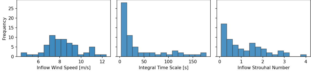
FIG. 5: Distributions of the average inflow wind speed, U_\infty , integral time scale, T , and Strouhal Number, St_{in} , at hub height for the subset of conditions corresponding to the 65 selected cases.
