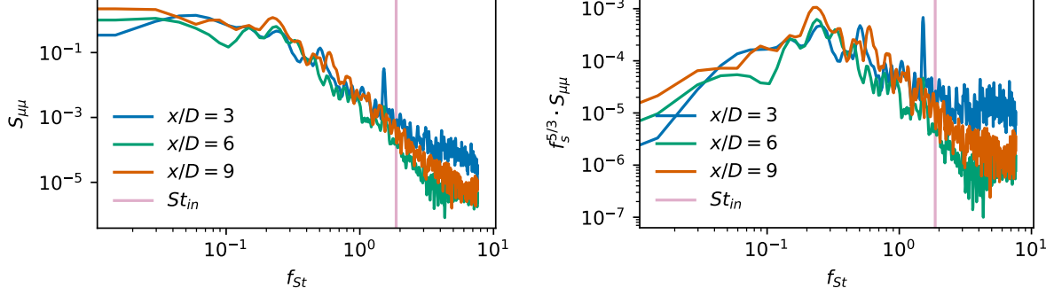
FIG. 12: PSDs (left) and premultiplied spectra (right) of detected wake centers from the lidar data at selected downstream distances.
