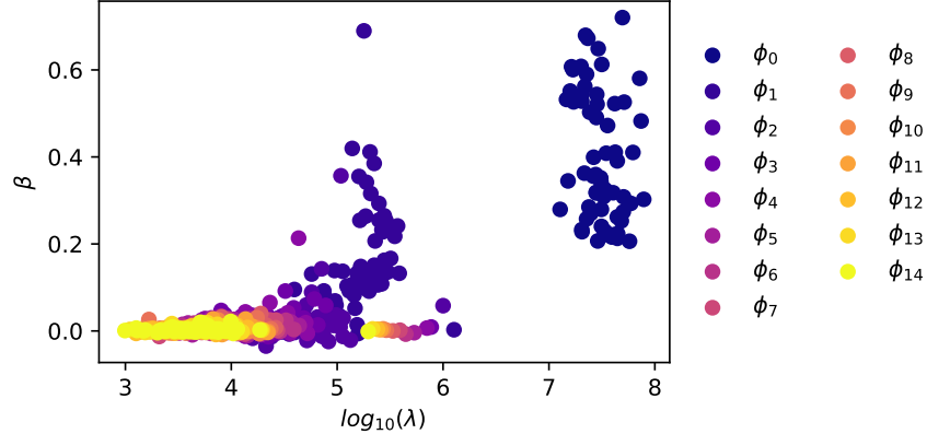
FIG. 25: Comparison of POD mode eigenvalues \lambda_i to main effect coefficients \beta_i for all 65 cases.
