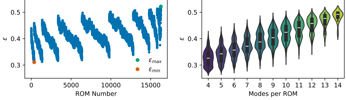
FIG. 18: Frequency and range-averaged coherence between detected wake centers from lidar scans and ROMs considering f_s \leq St_{in} Hz (left). Distribution of \varepsilon by the number of modes contained in each ROM (right).
