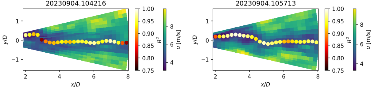
FIG. 10: Example lidar scans showing u overlaid with the fitted wake centers. Detected wake centers are colored by their respective coefficient of determination.
