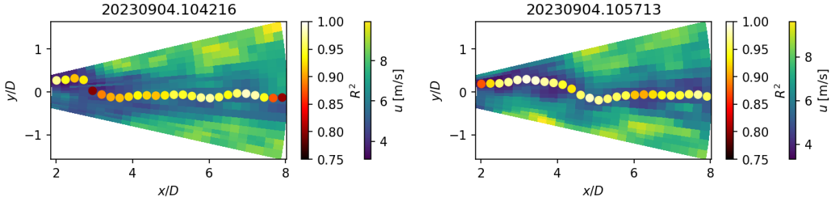
FIG. 11: Example lidar scans showing u overlaid with the fitted wake centers. Detected wake centers are colored by their respective coefficient of determination.
