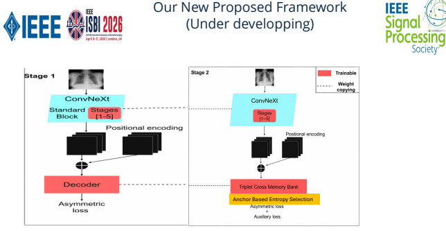
Fig. 1. Overview of the proposed Stage-2 fine-tuning pipeline. The Stage-1 ConvNeXt backbone and decoder are initialized from the frozen-free Stage-1 checkpoint and continue training with a Triplet Cross-Memory-Bank objective gated by Anchor-Based Entropy Selection, in place of the Mixture-of-Experts decoder used in our prior submission [12].
