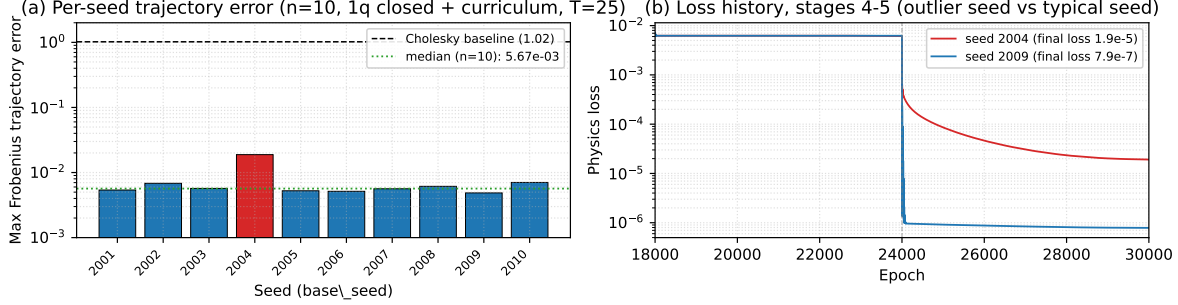
Figure 6: Multi-seed characterization of the 1q closed-system + curriculum result. (a) Per-seed max-Frobenius trajectory error across n = 10 seeds. Nine seeds cluster tightly near the median; seed = 2004 (red) is the outlier, still decreasing at the 30,000-epoch budget. Dashed line: Cholesky no-curriculum baseline (1.02). (b) Loss history for the outlier seed (2004) and a typical seed (2009) on curriculum stages 4-5. Both seeds are essentially identical through stage 4 (epochs 18,000–24,000); divergence emerges only in the final t_{\max} = 25 stage.
