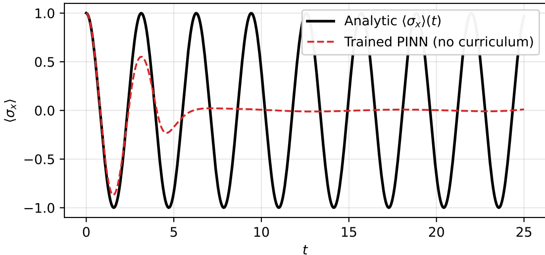
Local-vs-global gap: 1q closed-system, H = \sigma_z , IC |+\rangle\langle+|
