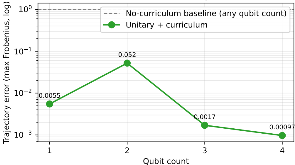
Curriculum closure across qubit count
