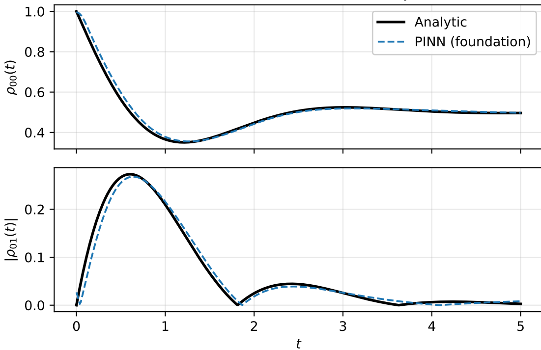
Foundation reproduction: 1q Lindblad, H = \sigma_y , L = \sigma_x , IC |0\rangle\langle 0|
