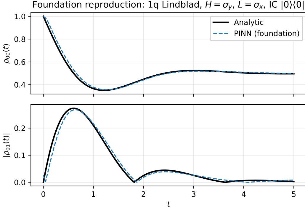
Figure 5: Foundation reproduction: cholesky-architecture PINN trained on the original 1-qubit Lindblad problem ( H = \sigma_y , L = \sigma_x with \gamma = 1 implicit, IC = |0\rangle\langle 0| , T = 5 ). The model’s population \rho_{00}(t) and coherence |\rho_{01}(t)| track the analytic Lindblad solution within \sim 6\text{--}9\% Frobenius error.
