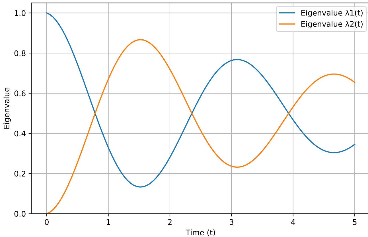
Eigenvalue evolution of \rho(t)
