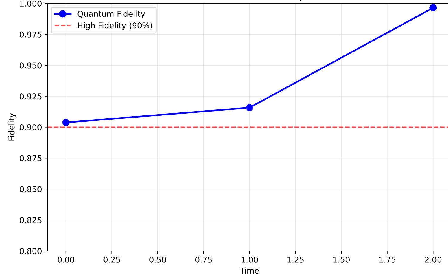
Quantum State Fidelity
