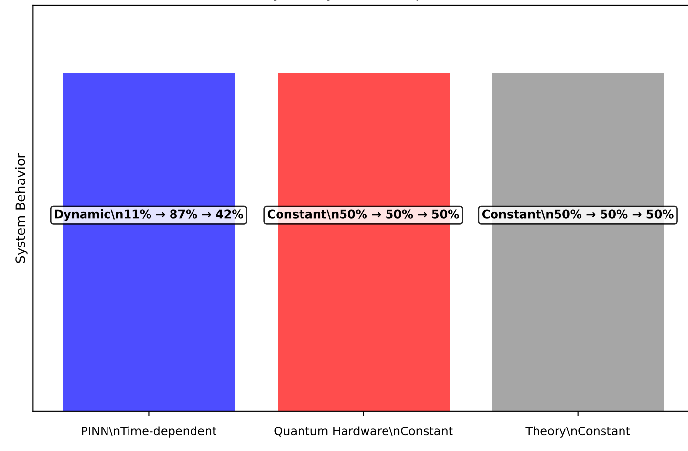
Physics System Comparison
