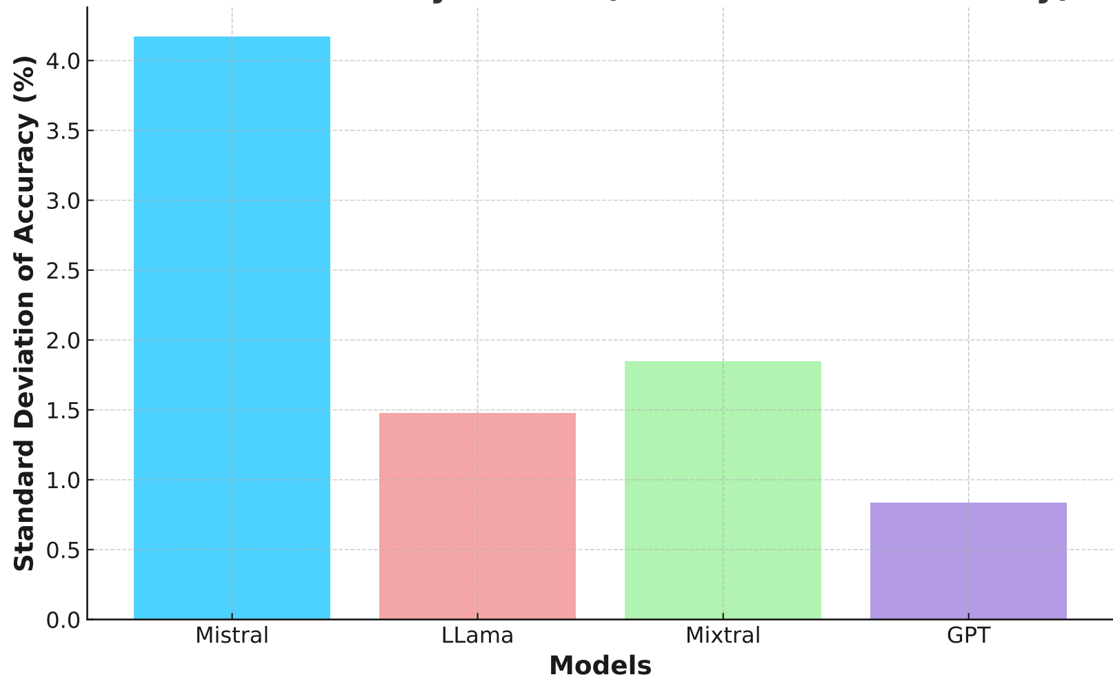
Model Sensitivity to Bias (Fluctuation in Accuracy)
