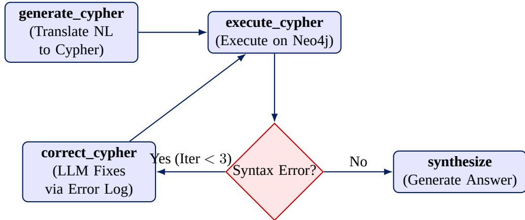
Figure 5.1: LangGraph State Machine for Self-Correcting Cypher Queries
