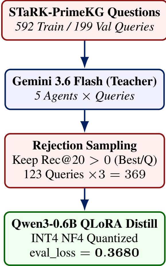
Figure 2: Trajectory Mining and Distillation Flow. Gemini 3.6 Flash teacher exploration with Rejection Sampling produces high-quality training trajectories for distilling Qwen3-0.6B.
