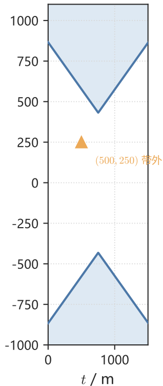
(c) 蝶形斜带 |h| \geq 包络
