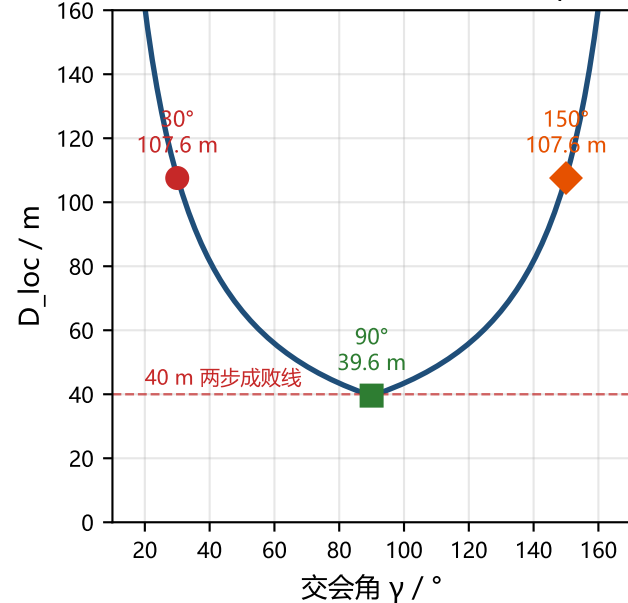
(c) d_1 = d_2 = 800 m 时直径随 \gamma
