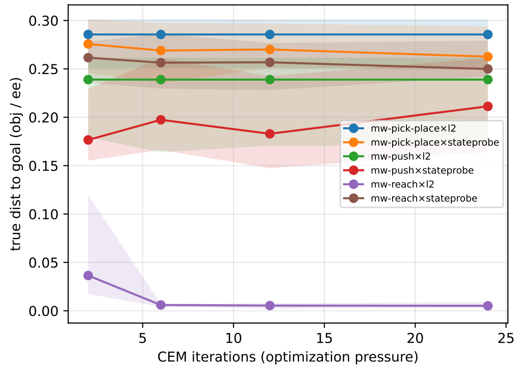
(A) Does more search help? (n=100 samples)
