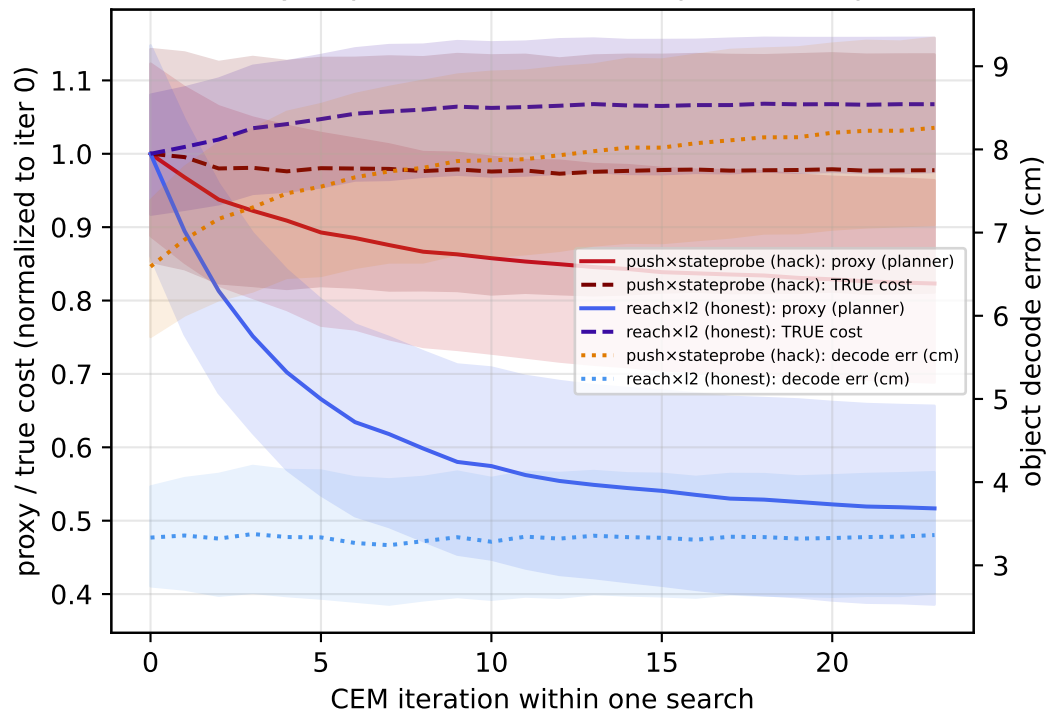
(B) Proxy improves, TRUE stalls, pocket deepens
