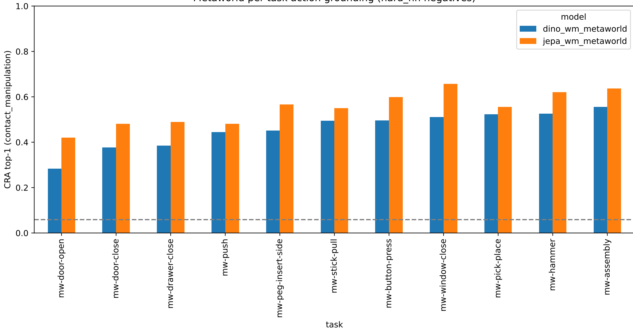
Metaworld per-task action grounding (hard_nn negatives)
