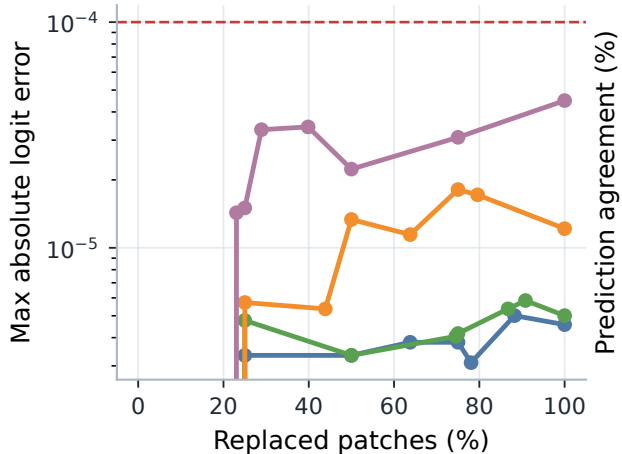
(a) Numerical discrepancy
