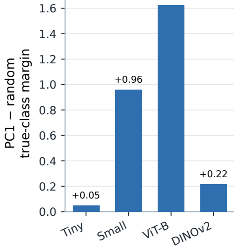
(b) PC1 advantage over random
