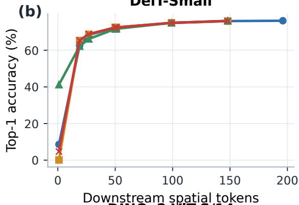
DeiT-Small
