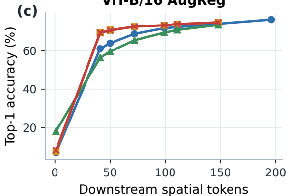
ViT-B/16 AugReg
