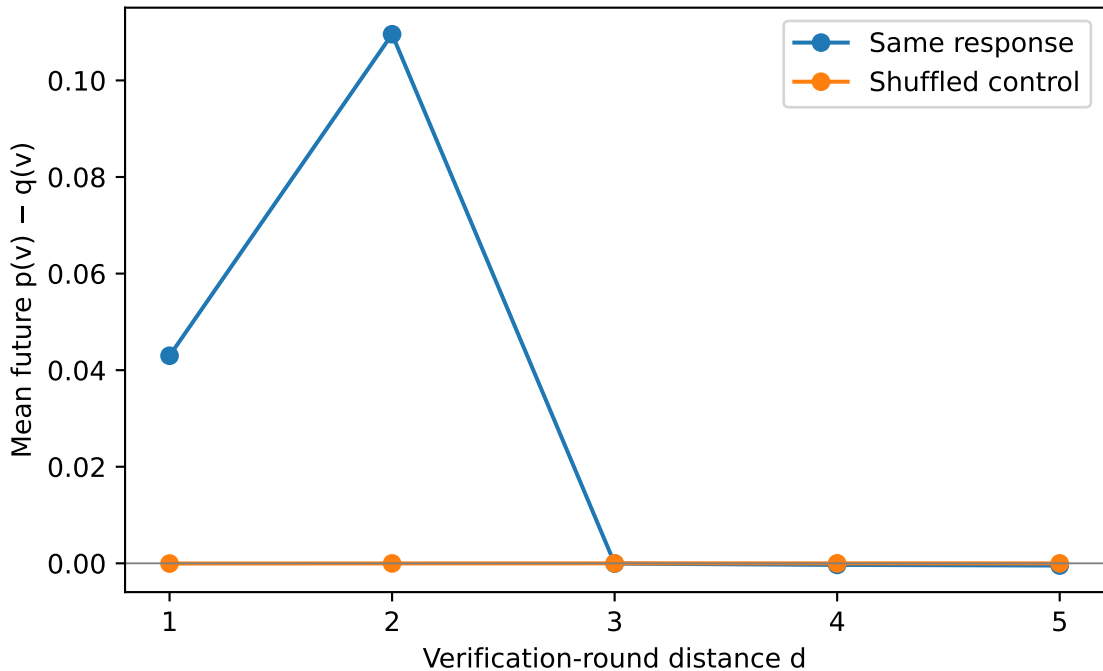
Root prediction-error persistence (paired contexts)
