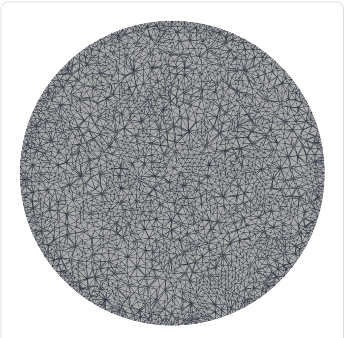
The conductor alone , 98,204 tets of the 179,477. Note it is uniform — no grading toward the axis, which is the decision argued for in §3.2 — and that at N = 76 the polygon is already visually a circle.
