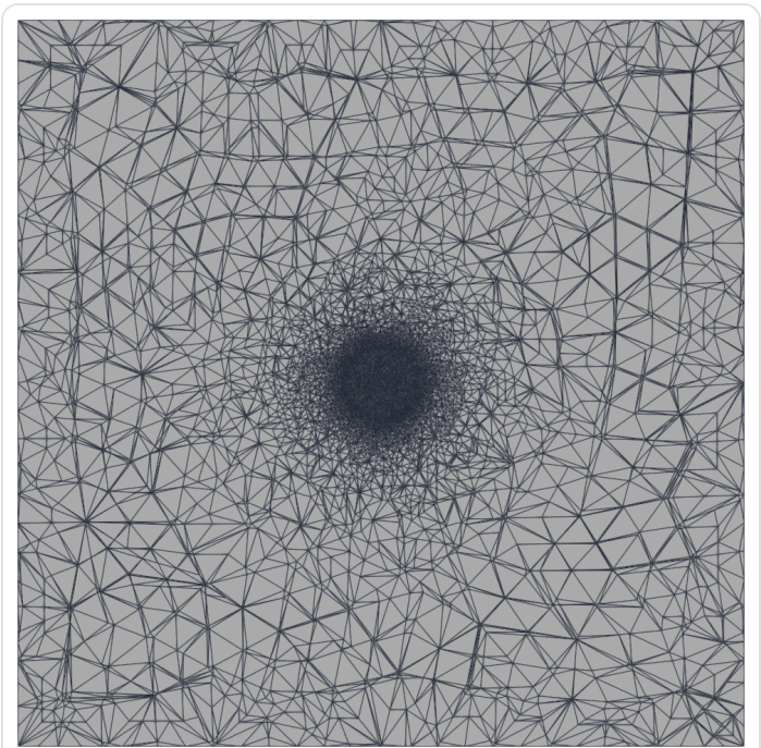
Whole domain , the 200 mm box at mid height. Graded from the conductor out to lc\_far = 16\text{ mm} at the wall over d\_far = 45\text{ mm} . The dark disc in the middle is the conductor and the shell of air around it, both held at the fine size.
