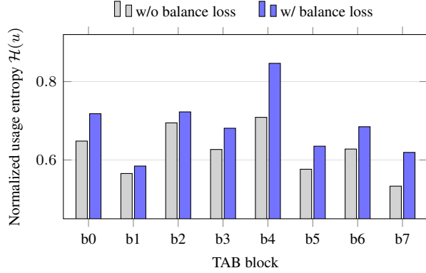
Figure 5. Normalized prototype-usage entropy \mathcal{H}(u) (Eq. (13); higher = more balanced) per TAB block ( b_0 – b_7 ) at \times 4 , iter 80k on Urban100. The usage-balancing regularizer increases the entropy in all eight blocks (block-mean 0.6227 \rightarrow 0.6865 ), confirming that it counteracts the collapse onto a few prototypes encouraged by the learnable temperature (C4).
