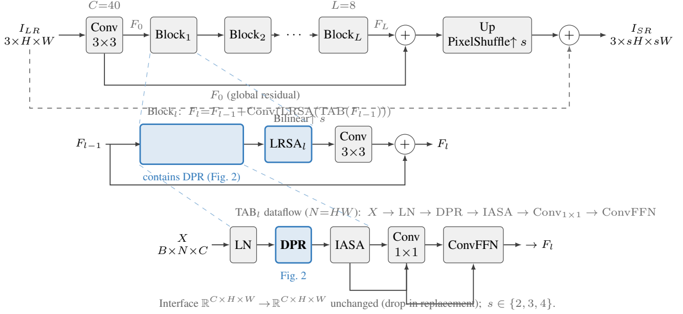
Figure 1. Overall architecture of DPRNet. A 3 \times 3 convolution extracts shallow features F_0 ( C=40 ); a stack of L=8 blocks, each coupling a Token Aggregation Block (TAB) with local self-attention (LRSAL) and a fusion convolution under a residual connection (Eq. (4) context, Eqs. (1)–(3)), produces F_L ; a global residual, a pixel-shuffle upsampler and a bilinear bypass reconstruct I_{SR} . The contribution is confined to the DPR module inside each TAB (highlighted), whose data flow X \rightarrow \text{LN} \rightarrow \text{DPR} \rightarrow \text{IASA} \rightarrow \text{Conv}_{1 \times 1} \rightarrow \text{ConvFFN} keeps the TAB interface \mathbb{R}^{C \times H \times W} \rightarrow \mathbb{R}^{C \times H \times W} unchanged, so the rest of the CATANet backbone is a drop-in host; DPR is detailed in Fig. 2.
