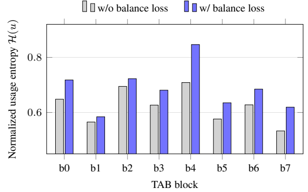
Figure 6. Normalized prototype-usage entropy \mathcal{H}(u) (Eq. (13); higher = more balanced) per TAB block ( b_0\text{--}b_7 ) at \times 4 , iter 80k on Urban100. The usage-balancing regularizer increases the entropy in all eight blocks (block-mean 0.6227 \rightarrow 0.6865 ), confirming that it counteracts the collapse onto a few prototypes encouraged by the learnable temperature (C4).
